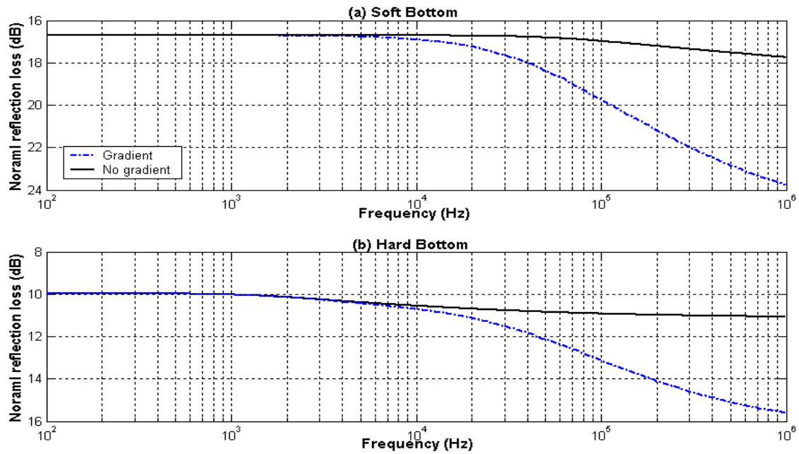
Fig. 4. The normal reflection loss versus frequency for soft and hard bottom .
