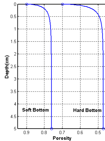
Fig. 1. The depth-porosity profile.
