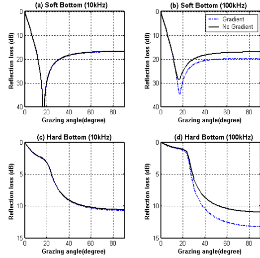
Fig. 3. The reflection loss versus the grazing angle at two frequencies for soft and hard bottom.
