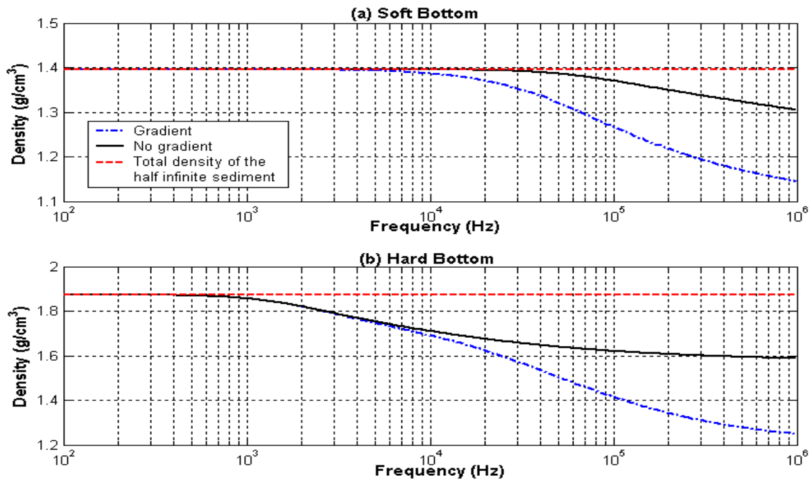
Fig. 5. The apparent density estimated from the normal reflection loss versus frequency for soft and hard bottom.
