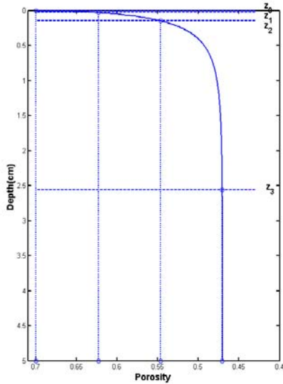
Fig. 2. The Example of the division of sediment layer.
