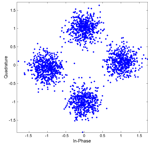
Fig. 6 Constellation of the received QPSK modulated signal after compensation for Doppler spread and time-delay spread for all paths
