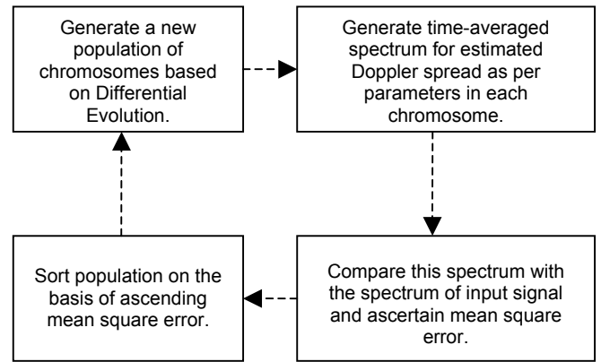
Fig. 2. Schematic block diagram for Doppler spread estimation using Differential Evolution.
