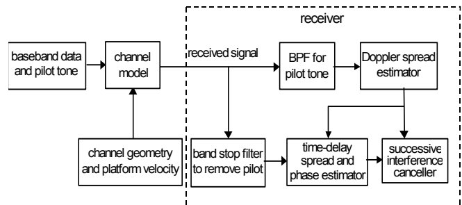
Fig. 1 Schematic block diagram of the communication system
