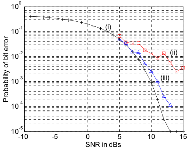
Fig. 7 Effect of the SNR on the bit error probability of the underwater acoustic communications system for channel model of Table II using the original channel estimator: (i) AWGN, (ii) compensation for the Doppler on the dominant path only, (iii) compensation for Doppler spread and time-delay spread.
