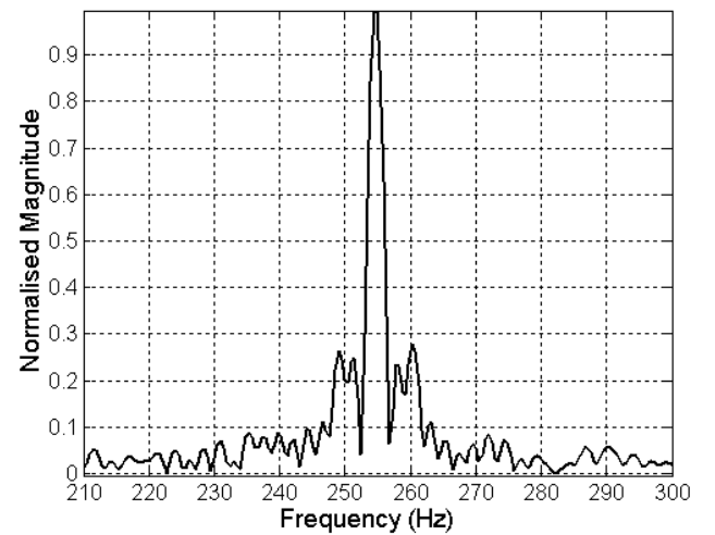
Fig. 3. Spectrum showing the three Doppler shifted/spread paths with spurious peaks at an SNR=12dB.
