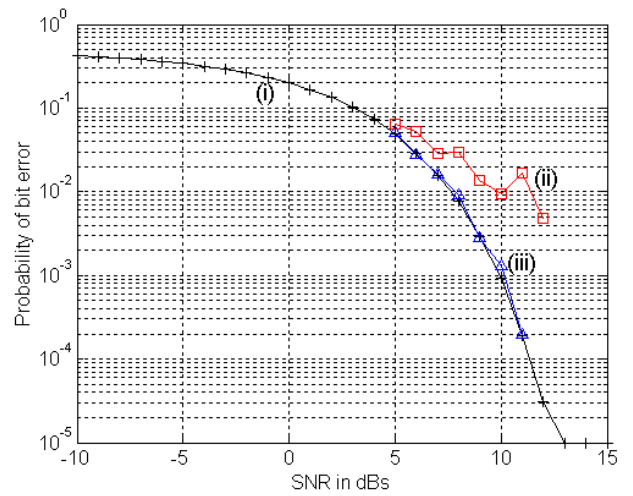
Fig. 8. Effect of the SNR on the bit error probability of the underwater acoustic communications system for channel model of Table II using the new channel estimator: (i) AWGN, (ii) compensation for the Doppler on the dominant path only, (iii) compensation for Doppler spread and time-delay spread.
