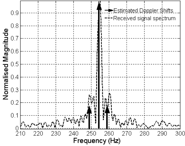
Fig. 4. Estimated Doppler shifts superimposed on the received spectrum
