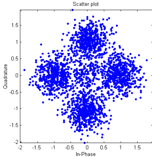
Fig. 5 Constellation of the received QPSK modulated signal after correction for only the Doppler on the dominant path
