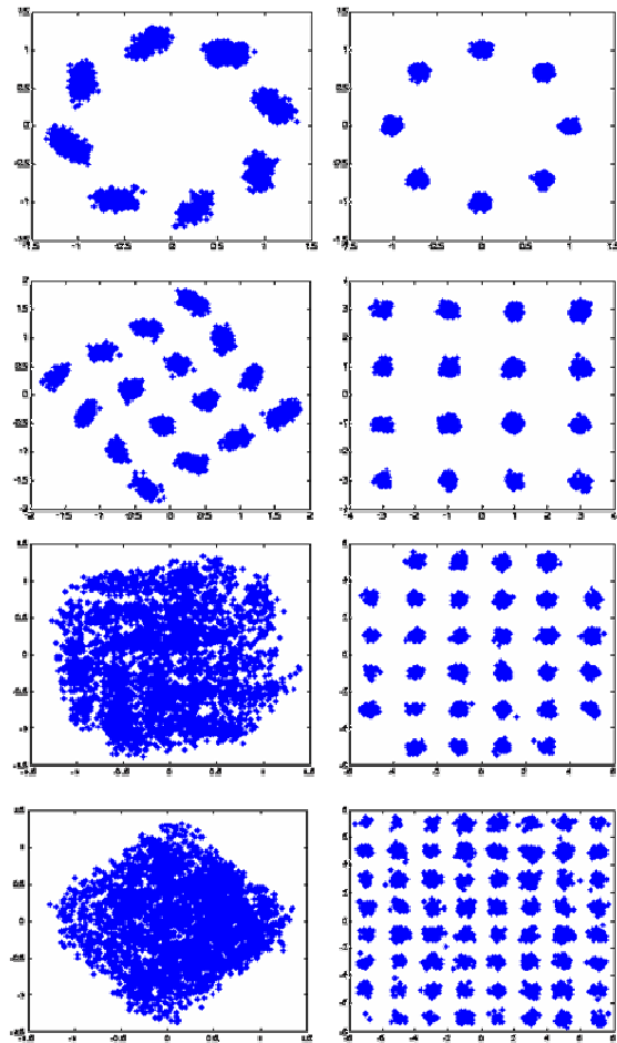
Fig. 6. Scatter plots of 8-PSK, 16-QAM, 32-QAM and 64-QAM, before and after equalization using an 11 tap linear LMS equalizer.
