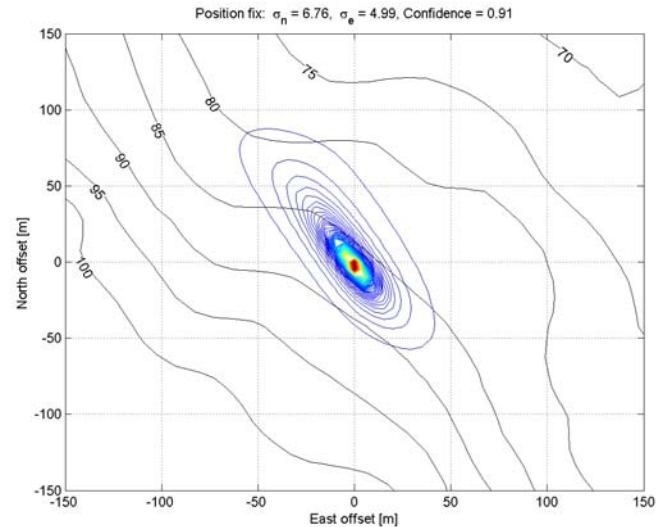
Fig. 10. The correlation surface contour lines overlaid the DTM contour lines for a 300m x 300m area. HUGIN I's position estimate (considered true position) is in the origin of this grid. Notice that the uncertainty of the fix is greater in the direction along the contour lines than across, indicating the importance of the position fix covariance.
