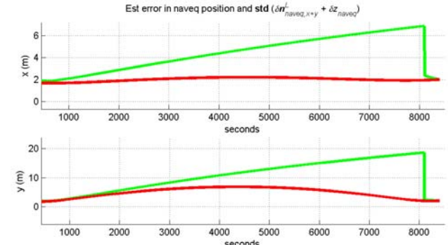
Fig. 4. The effect of navigation post-processing when running a straight trajectory with GPS fix every 15 km. Green graph: real-time position accuracy ( 1\sigma ). Red graph: post-processed position accuracy ( 1\sigma ). x and y in local level (L) corresponds roughly to North and East direction.
