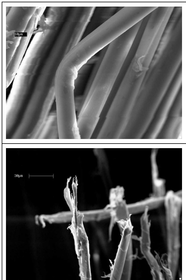
Figure 5: Bent fiber from an outer strand showing compression bands (above) and a fiber from the core, broken in tension, with no sign of fibrillation (below) during bend-over-sheave testing of an unbalanced rope with one end free to rotate.
