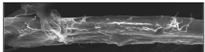
Figure 4: SEM image of a fiber showing crushing near its center.
