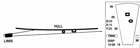
Fig. 3. The LIMIS is held near the hull to get a small grazing angle. Targets are displayed as if seen from below with a sound source illuminating the target from the side.
