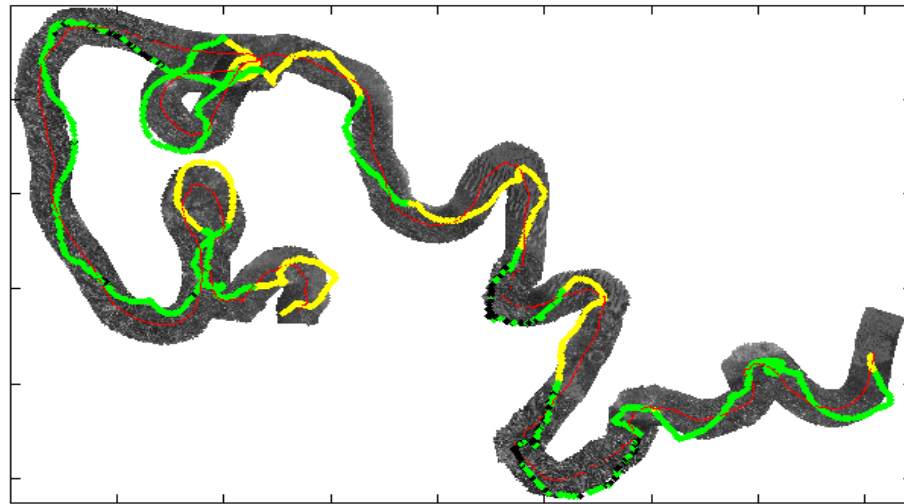
Figure 6: classification ( N=32 ).
