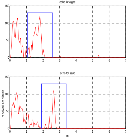
Figure 3: Profiles received from Posidonia (top) and sand (bottom) during one experiment at sea.
