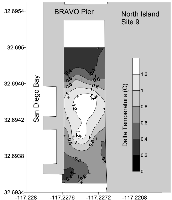
Fig. 14. Spatial distribution of the temperature contrast between near bottom and sub-bottom temperature at 60 cm depth.
