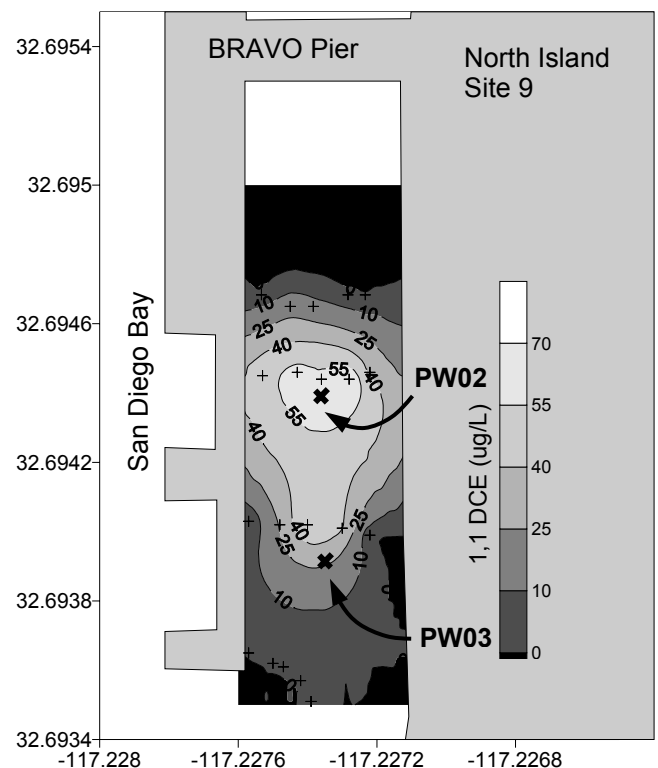
Fig. 15. Spatial distribution of DCE concentration.
