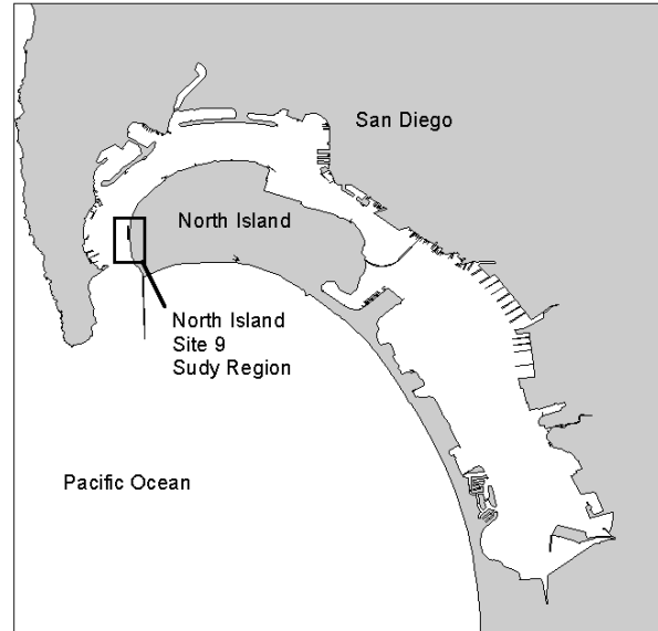
Fig. 12. Map of San Diego Bay and the study region.
