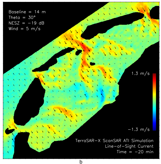
Fig. 11. Simulated TerraSAR-X ScanSAR mode data products for the "Waddenzee" scenario; (a) split antenna configuration, effective time lag = 0.17 ms; (b) proposed dual antenna / boom configuration, effective time lag = 2 ms.
