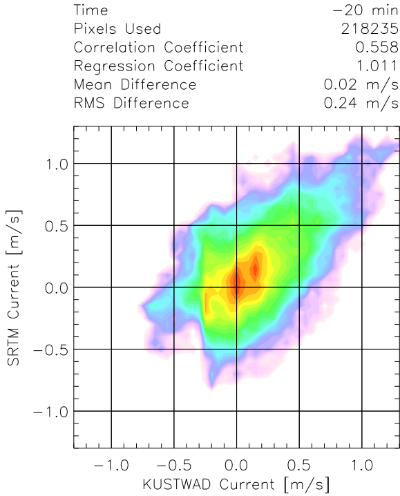
Fig. 6. Scatter diagram showing the distribution of SRTM-derived vs. KUSTWAD-derived current components in the SRTM look direction, as well as corresponding statistical quantities, for the tidal phase 20 minutes before the SRTM overpass.
