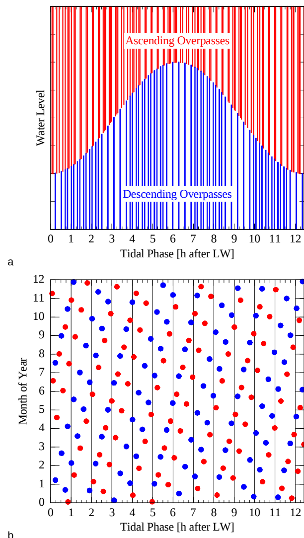
Fig. 10. Coverage of the tidal cycle in the Waddenzeer by ascending and descending TerraSAR-X overpasses within a period of one year; (a) total coverage; (b) coverage at different times of the year.
