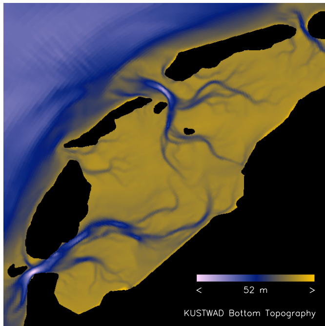
Fig. 4. Bottom topography of the circulation model KUSTWAD in the 70 km \times 70 km "Waddenze" test area.
