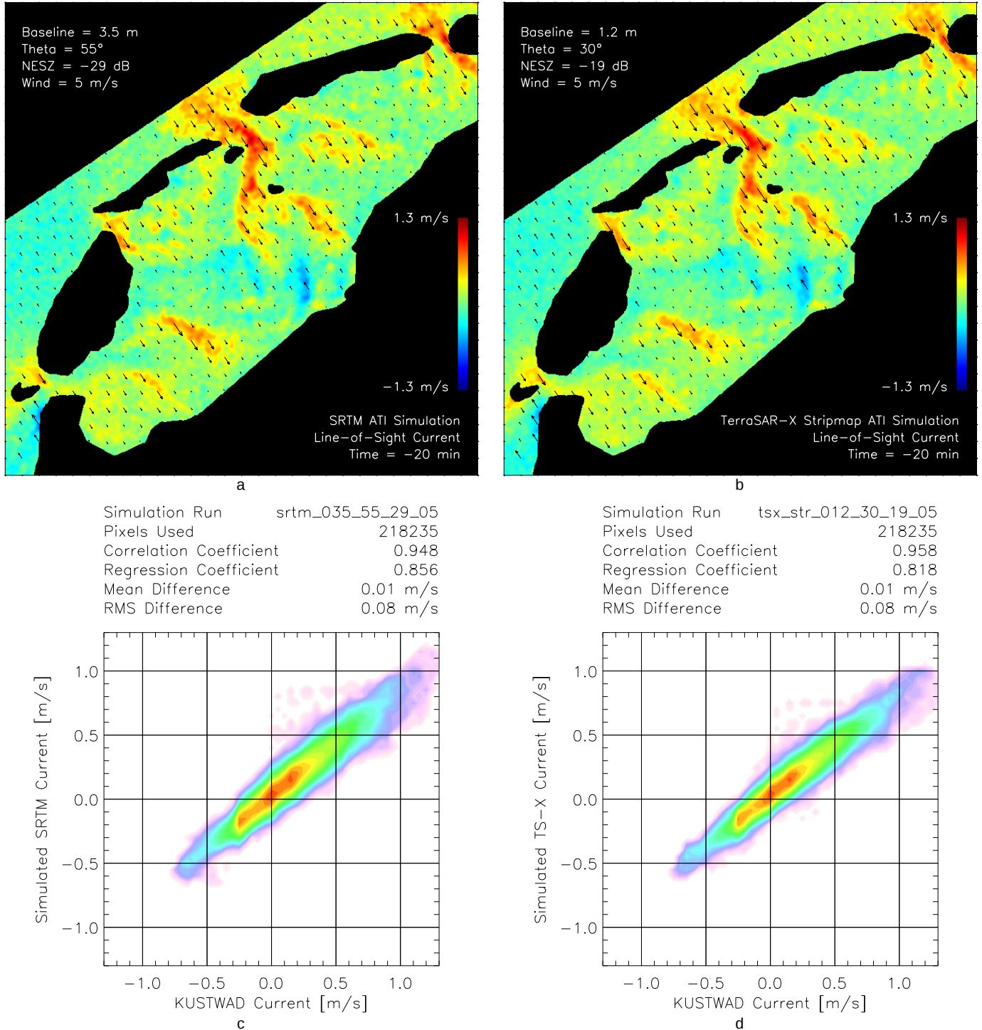
Fig. 9. Simulated InSAR-derived line-of-sight current fields for the SRTM swath in the "Waddenzee" scenario and statistical diagrams; (a) SRTM simulation result; (b) TerraSAR-X stripmap mode simulation result; (c) distribution of SRTM simulation results vs. KUSTWAD currents and statistical parameters; (d) distribution of TerraSAR-X simulation results vs. KUSTWAD currents and statistical parameters.
