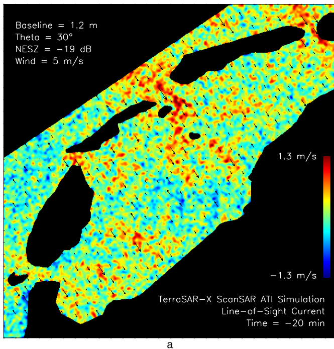
Fig. 11. Simulated TerraSAR-X ScanSAR mode data products for the "Waddenzee" scenario; (a) split antenna configuration, effective time lag = 0.17 ms; (b) proposed dual antenna / boom configuration, effective time lag = 2 ms.
