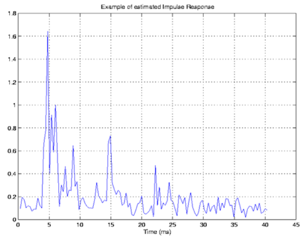
Figure 6 – An example of measured channel impulse response
