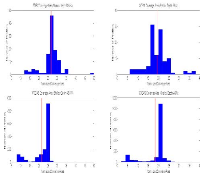
Fig. 8. Shallow depth band coverage percentage distributions: upper panels for GDEM and lower panels for MODAS, left panels for ASUW scenario and right panels for ASW scenario.
