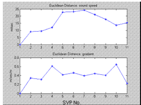
Figure 4. Euclidean distance metric for Korea Straits profiles. A measure of dissimilarity between profiles.
