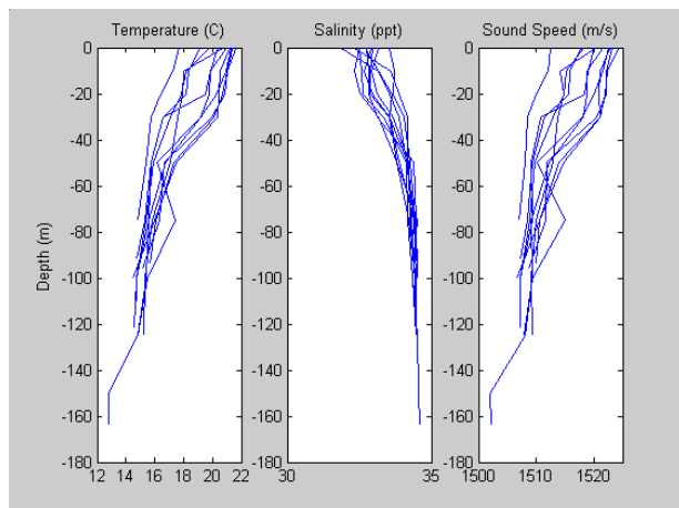
Figure 3. Temperature, salinity and derived sound speed profiles for Korea Straits environment.
