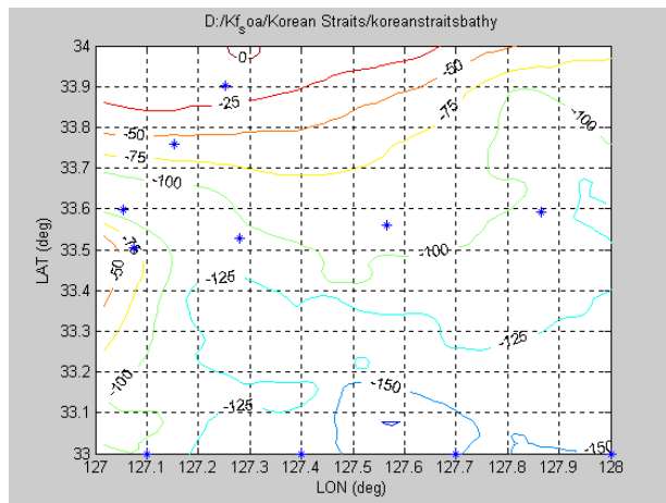
Figure 2. Geographic location of profile data used for Korea Straits environment (bathymetric contours in meters).
