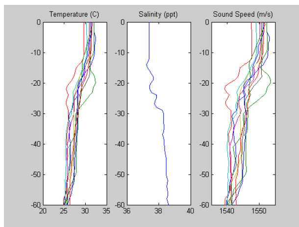
Figure 6. Temperature, salinity and derived sound speed profiles for Straits of Hormuz environment.
