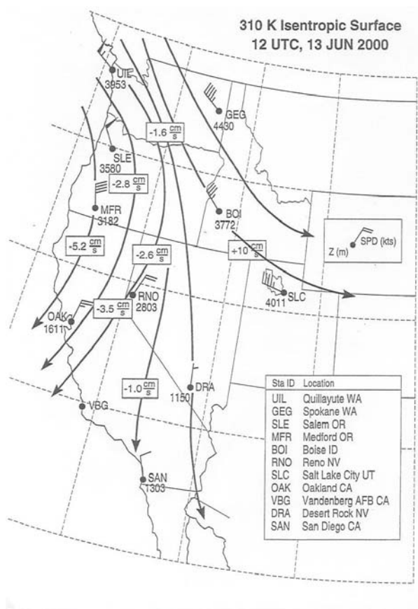
Figure 2. 310 K isentropic surface analysis valid 1200 UTC 13 June 2000.
