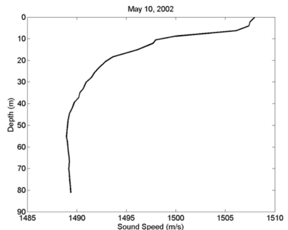
Fig. 3. Measured sound speed profile for SX-F site off the coast of San Diego on May 10, 2002.
