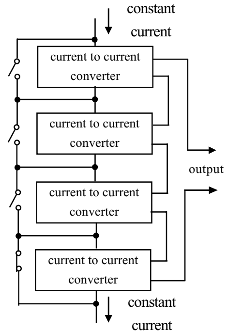
Fig.5 Typical configuration of a current source that will be placed in the PBU
