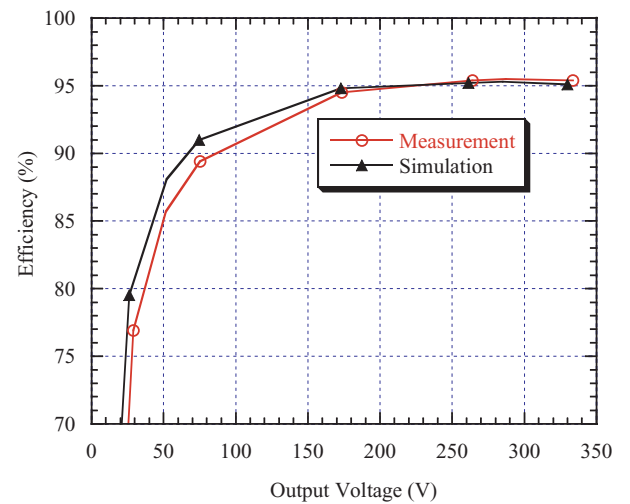
Fig.11 Efficiency of the current - current converter
