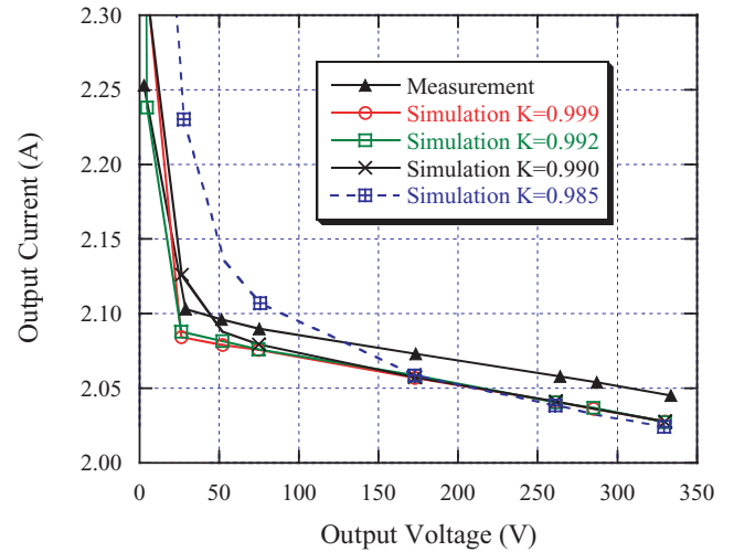
Fig.10 Load regulation calculated by computer simulation when changing coupling coefficient
