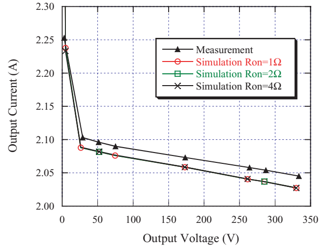
Fig.9 Load regulation calculated by computer simulation when changing on-resistance of FETs
