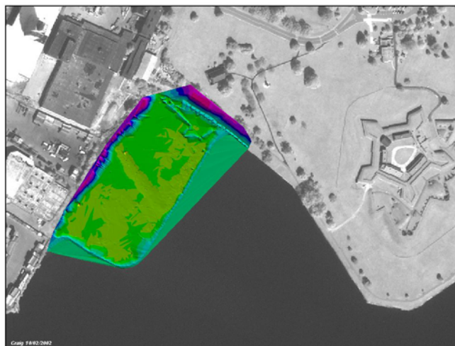
Fig. 3. Fort McHenry pre-construction Digital Elevation Model (DEM).
