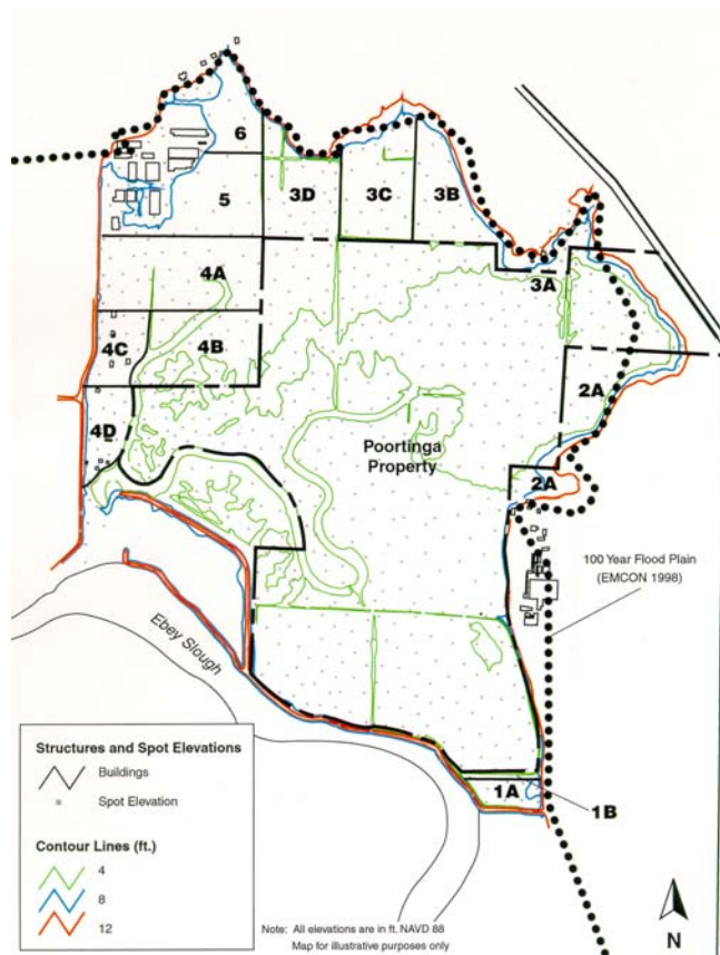
Fig. 6. Existing elevations at Qwuloolt Marsh site in Marysville, WA. Critical elevations are 4 ft, 8 ft, and 12 ft relative to NAVD88.
