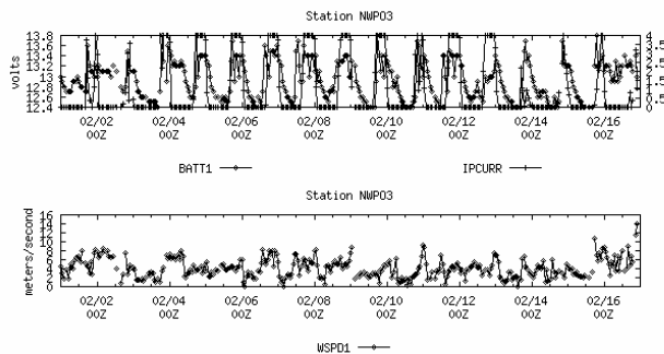
Fig. 7. Stacked time series plots of overlaid battery system voltage and solar charging current compared to wind speed month of February.
