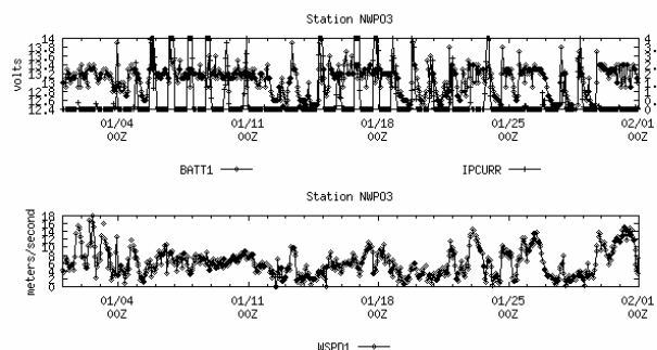
Fig. 6. Stacked time series plots of overlaid battery system voltage and solar charging current compared to wind speed month of January, 2003.
