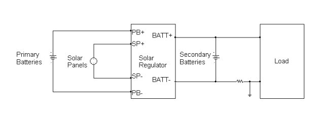
Fig. 1. Block diagram of present NDBC C-MAN power.
