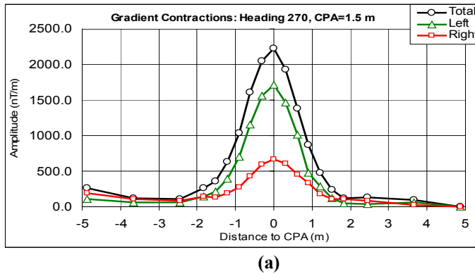
Fig. 6. Gradient contraction and total field data for a tangential approach to the target on a heading of 270^\circ (path 3 of Fig. 3(c)). The Left axis of the sensor system was closer to target than the Right axis and the magnitudes of the Left axis gradient contraction and total field sums are greater than the respective values for the Right axis.
