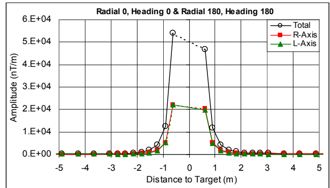
Fig. 9. Gradient contractions as the sensor system moved directly toward the target (to a CPA of 0.6 m) on radial paths of 0° and 180° (indicated by the vertical arrows in Fig. 3 (a)).
