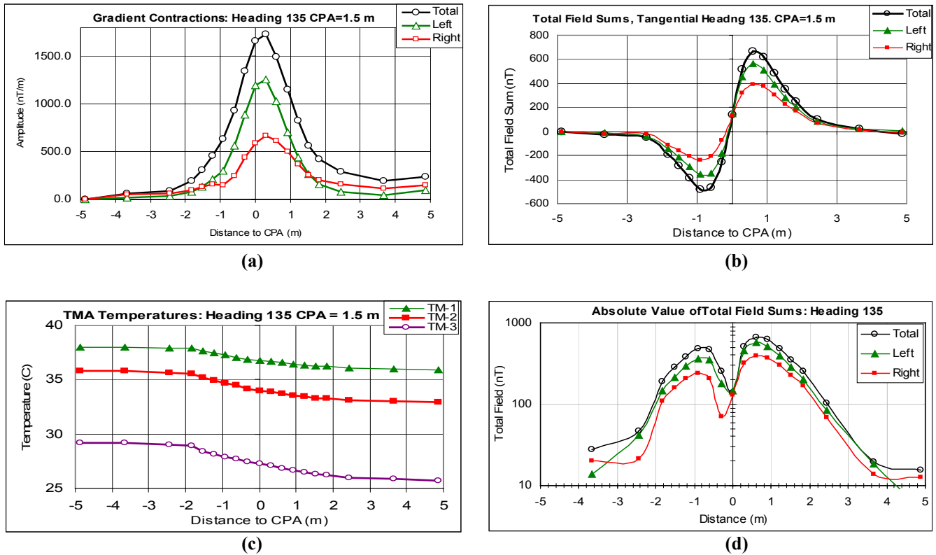
Fig. 4. Gradient contraction, total field and temperature data for the sensor system on a tangential approach to the target with a heading of 135^\circ (path 6 of Fig. 3(c)). For these data curves, the left axis of the sensor system was closer to target than the right axis.
