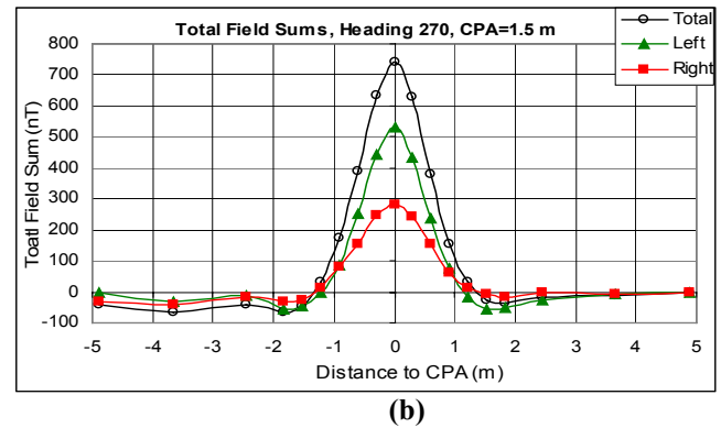
Fig. 6. Gradient contraction and total field data for a tangential approach to the target on a heading of 270^\circ (path 3 of Fig. 3(c)). The Left axis of the sensor system was closer to target than the Right axis and the magnitudes of the Left axis gradient contraction and total field sums are greater than the respective values for the Right axis.
