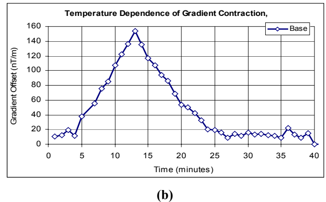
Fig. 7. Correlation of TMA temperature and gradient contraction output drift. The gradiometer sensor was fixed on a heading of 0^\circ with no target present and TMA-2 of the base axis was cooled for about 7 minutes. Part(a) shows the TMA temperature and Part (b) the corresponding variation in the Base axis gradient contraction, C_B .
