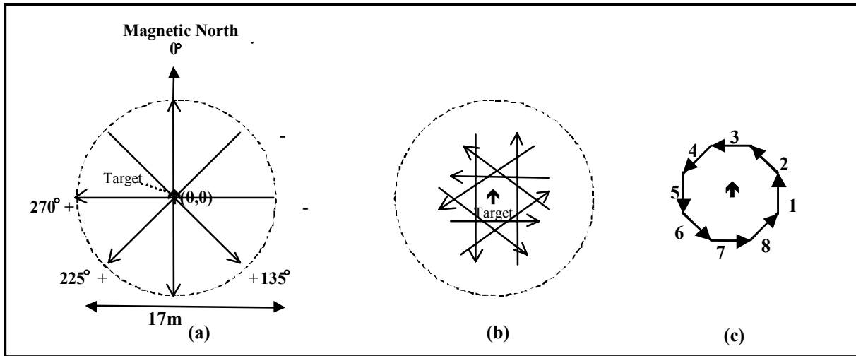
Fig. 3. Sketch of test range for gradiometer field tests. A permanent magnet dipole target with moment |\mathbf{M}| = 14.5 \text{ Am}^2 and with declination of 0^\circ and inclination 19^\circ was fixed at the center (0,0) of the 17m diameter range. Data were taken by moving the sensor along the paths indicated by arrows in (a)–(c). Part (a) represents "radial" approaches to target with the sensor path passing through the target position, while (b) shows "tangential" approaches to within 1.5 m from the target. Part (c) represents the two-dimensional closure of the tangential paths around target. For the eight tangential paths of (b),(c) the sensor system's Left Guidance Axis was closer to target than the Right Axis. Within the gradiometer detection range, the magnitude of Left-Axis gradient contraction C_L was larger than that of the Right Axis's C_R for all eight paths.
