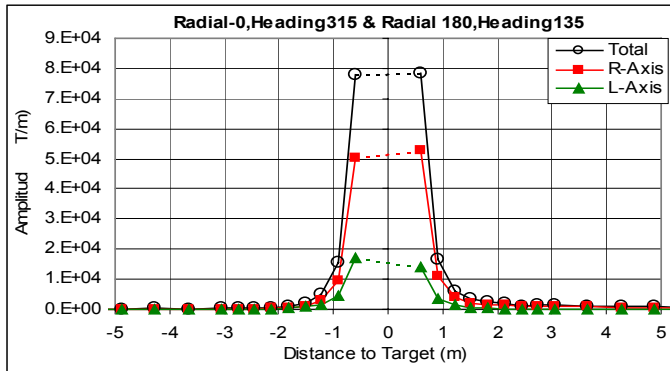
Fig. 9. Gradient contractions as the sensor system moved directly toward the target (to a CPA of 0.6 m) on radial paths of 0° and 180° (indicated by the vertical arrows in Fig. 3 (a)).
