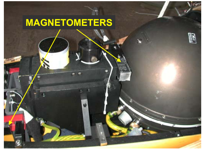
Figure 12. Port magnetometer relocation
