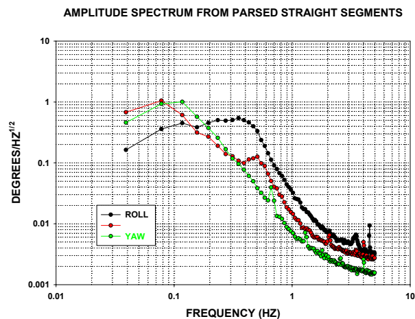
Figure 4. Roll, pitch and yaw amplitude spectra
