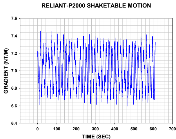
Figure 5. P2000-RELIANT raw gradient during motion
