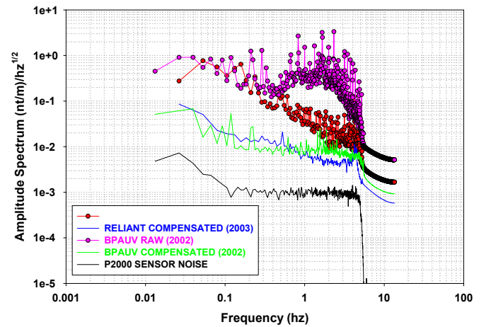
Figure 9. Raw and compensated amplitude spectra
