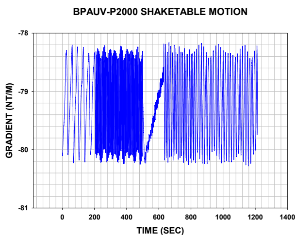
Figure 2. P2000-BPAUV raw gradient during motion
