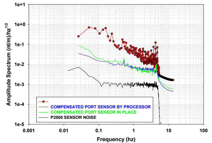
Figure 13. Residual for new magnetometer location
