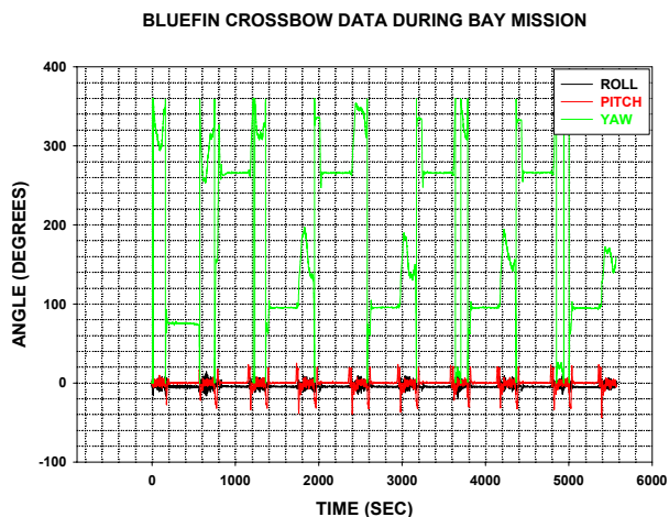
Figure 3. Mission roll, pitch and yaw
