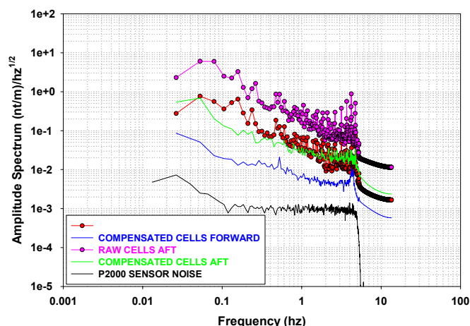
Figure 16. Two sensor positions compared
