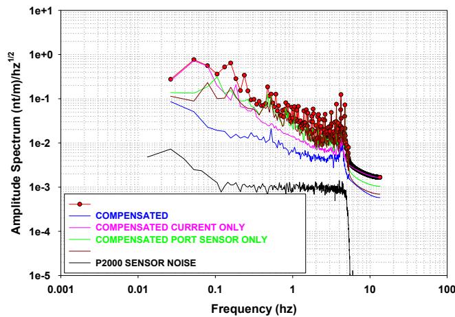
Figure 10. Removal of any one reference sensor
