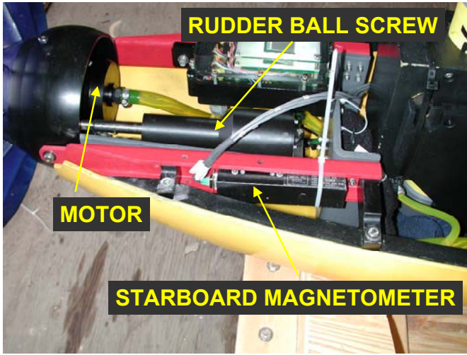
Figure 7. Reference magnetometer location
