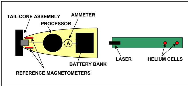
Figure 8. Schematic of vehicle-sensor layout
