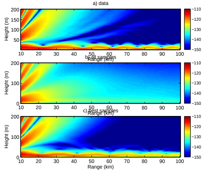
Fig. 5. The propagation-loss field based on (a) the true environment (from Fig. 3a), based on (b) prior information, and (c) posteriori information (bottom).
