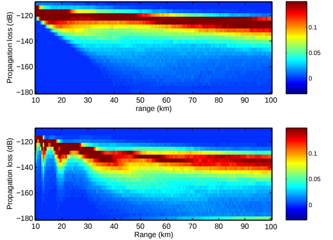
Fig. 6. Prior probability distribution for propagation loss versus range at 10 m (top) and 100 m (bottom) height.
