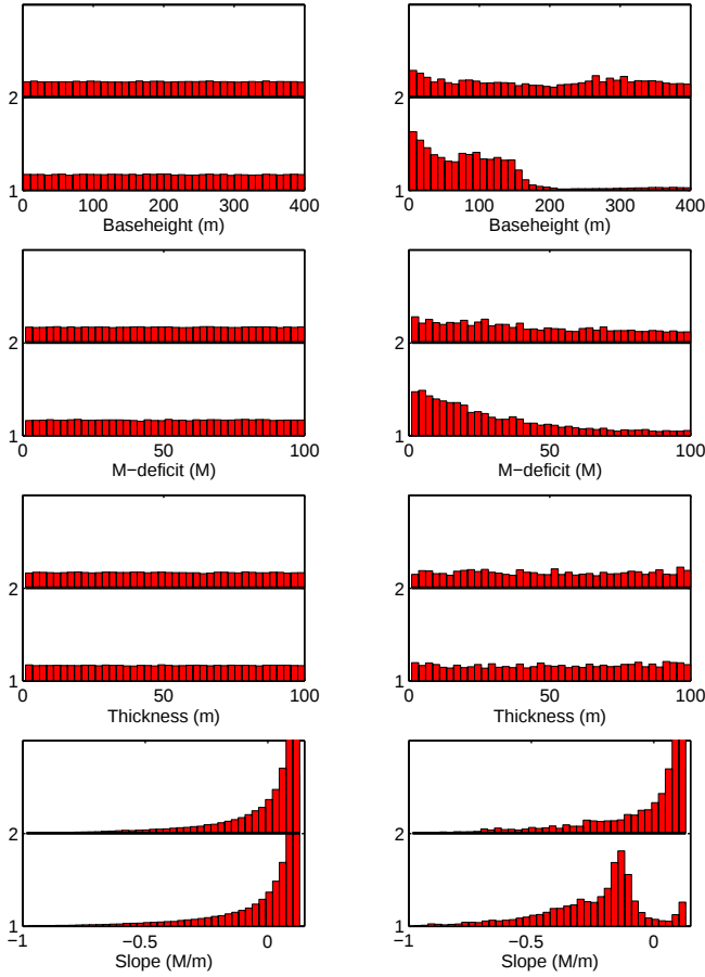
Fig. 4. Prior (left) and posteriori (right) distributions of the parameter estimates.
