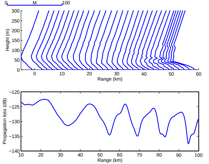
Fig. 3. The refractivity profile (a) used to generate the data, and (b) the propagation loss data.
