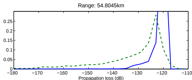
Fig. 8. Posteriori (solid) and prior (dashed) probability at 50 km range and 10 m height.
