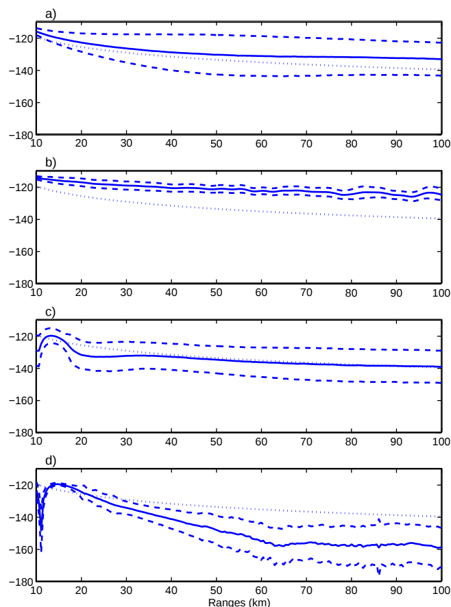
Fig. 9. The average field (solid) and plus/minus one standard deviation (dashed) based on all prior samples (a and c) and just the best posteriori samples (b and d) at 10-m height (a and b) 100-m height (c and d). For reference a r^{-1} decay (dotted) is shown on each plot.
