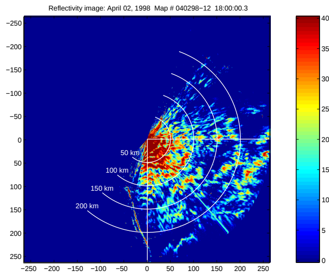
Fig. 1. Clutter map from SPANDAR corresponding to Wallops Run 12.
