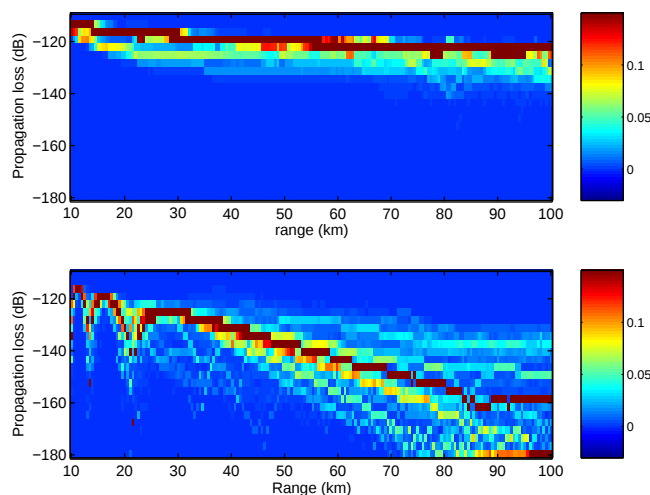
Fig. 7. Posteriori probability distribution for propagation loss versus range at 10 m (top) and 100 m (bottom) height.
