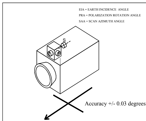
Fig. 3. Inclinometer mounting
