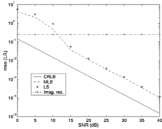
Fig. 6. Mse's of the MLE and LSE compared to the CRLB and imagin resolution for different SNR values and L/\lambda=1.667 (correlated reverberation with \gamma=3 ).
