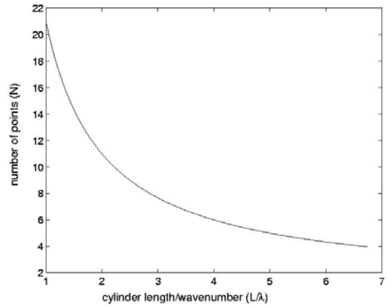
Fig. 3. Number of sampling points for different values of the normalized cylinder length L/\lambda .
