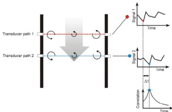
Fig. 3 Schematic representation of current measurement by acoustic scintillation
