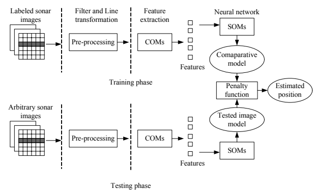
Fig. 1. Architecture of seabed recognition and detection system
