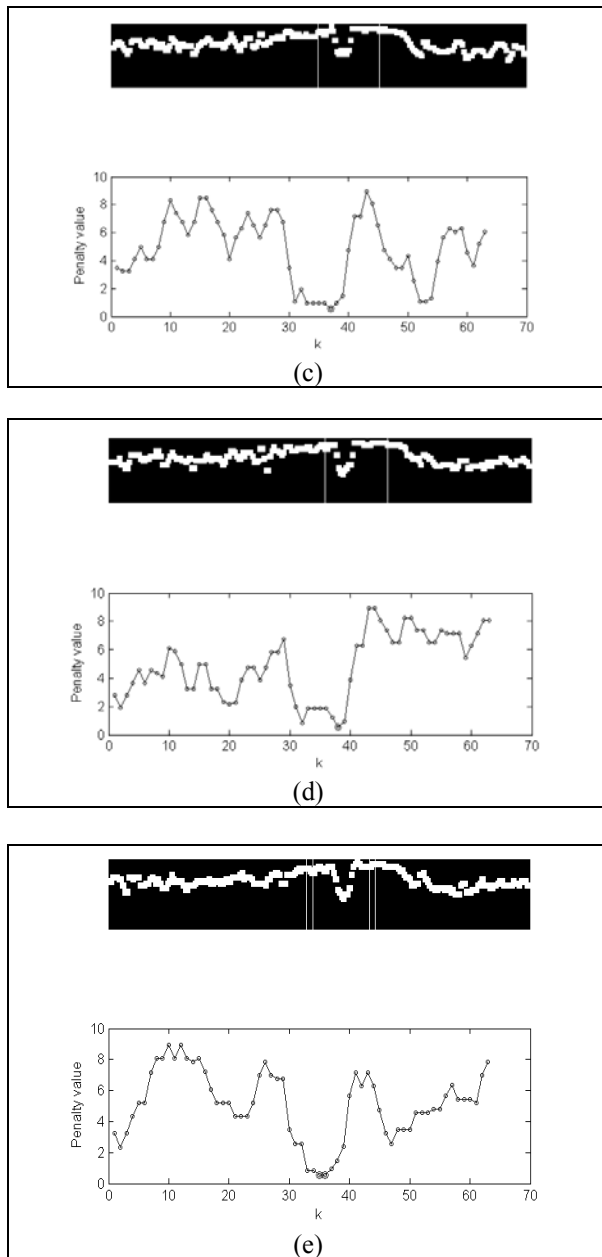
Fig. 15.(a-e). Each picture shows the pipeline position indicated by the best-matching window marked in the transformed line images above.
