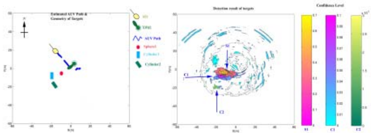
Fig. 6 Track and detection results, using 50 pings from the GOATS' 2000 experiment
