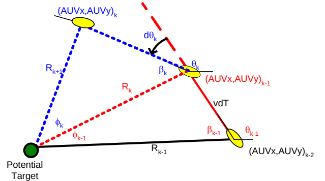
Fig. 4. Illustration of the relationship between state space of AUV and the beam space image: The fixed potential target shown in the figure are linked with AUV with the R and \beta in difference stage k .
