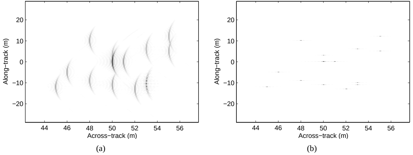
Fig. 1. Images containing a number of prominent points without sway: (a) magnitude of pulse-compressed echo history ss(u, t) , (b) magnitude of reconstructed image ff(x, y) .
