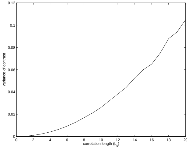
Fig. 9. Variance of contrast over several speckle patterns as a function of speckle correlation length L_c .
