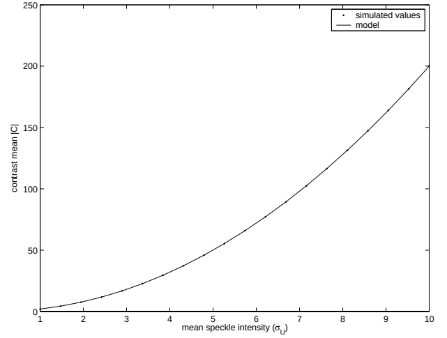
Fig. 6. The mean contrast for several speckle realisations as a function of the mean speckle intensity \sigma_U . It is compared against the model: E[C] = 2\sigma_U^2 .
