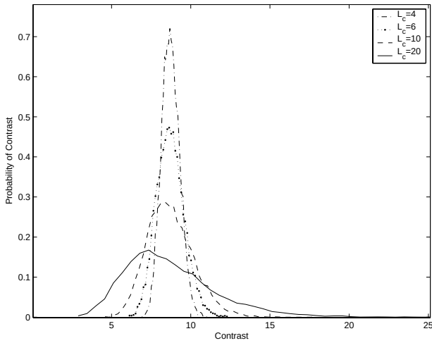
Fig. 8. Probability distributions of contrast for several simulated speckle patterns. Shown for varied correlation lengths, L_c = 4, 6, 10, 20 .
