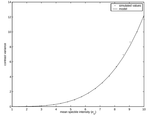
Fig. 7. The variance of the contrast for several speckle realisations as a function of the mean speckle intensity \sigma_U . It is compared against the model: \text{Var}[C] = 20\sigma_U^4/N .
