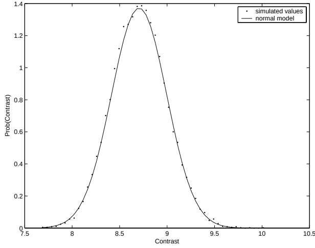
Fig. 5. Estimated probability distribution of contrast from simulated speckle. Data has mean and variance of \mu_C=8.7 \sigma_C^2=0.085 respectively. Data is compared against normal distribution model:
