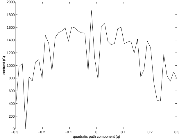
Fig. 2. Variation in contrast as a single focus parameter (quadratic towfish path component) is varied on a field SAS image.
