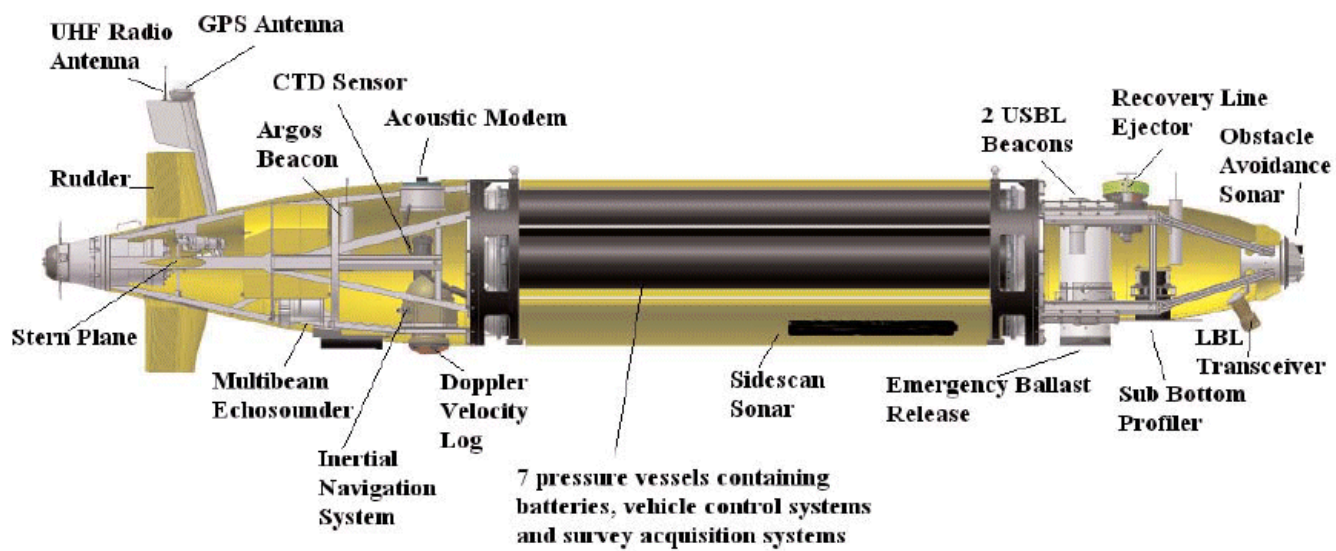
Fig. 12. Schematic overview of the Geosub's physical layout
