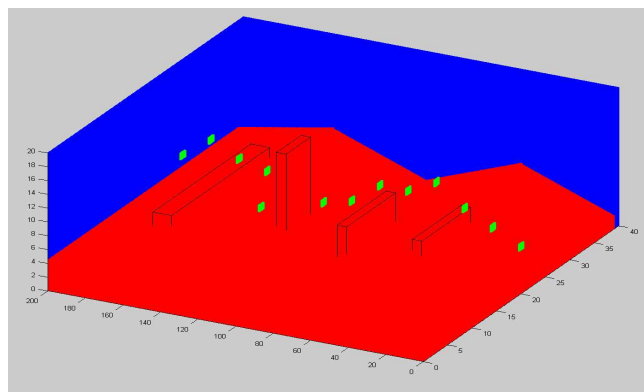
Fig. 7. Example of 3D obstacle avoidance, including "rise-over" motion.
