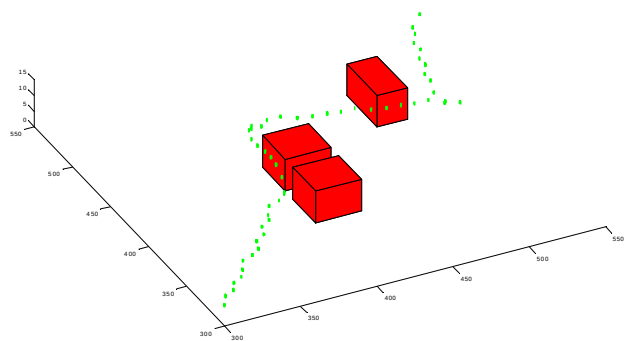
Fig. 8. Example of horizontal avoidance motion where vertical ascent is impossible.
