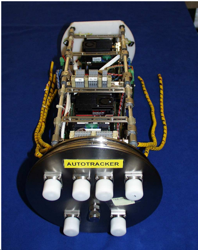
Fig. 10. Photograph of the AUTOTRACKER "pod" – with its four high-performance PC104-based computers (total length: ~55cm)
