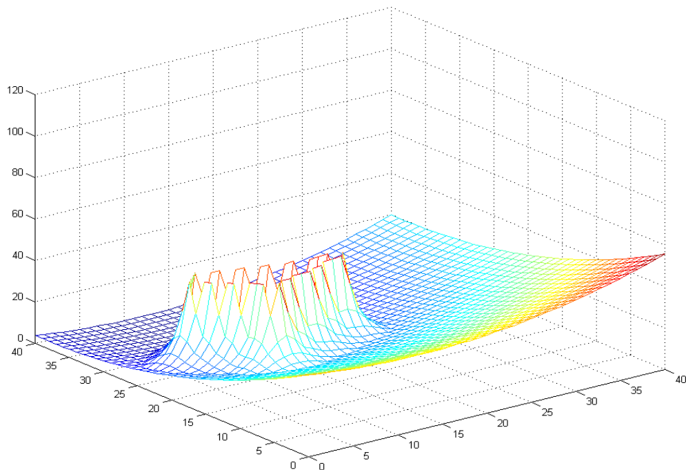
Fig. 4. 2-D potential well with obstacle - height indicates magnitude of potential.
