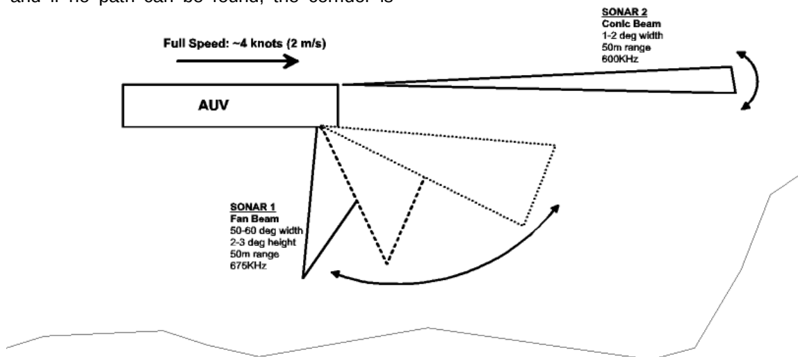
Fig. 3. The dual sonar configuration used for the 3D OAS and Path Planning system.
