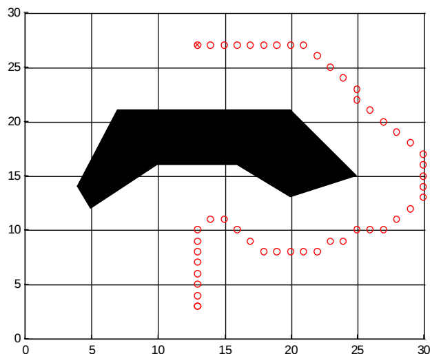
Fig. 6. Best first algorithm avoiding local minima.
