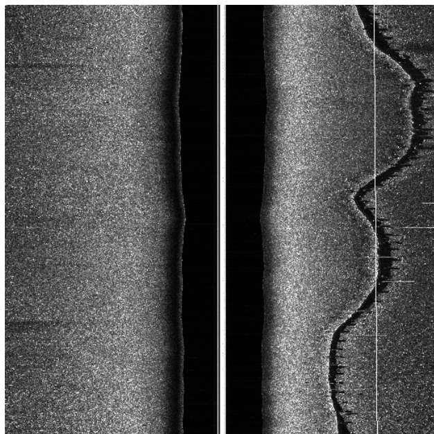
Fig. 1. Side-Scan image with detected trajectory.
