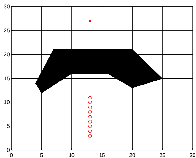
Fig. 5. Depth first algorithm trapped in local minima.
