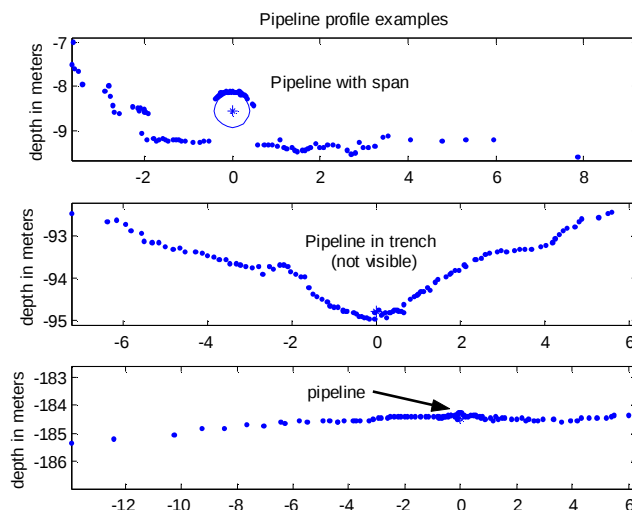
Fig. 2. Examples of raw MBE profiles for various different pipelines.
