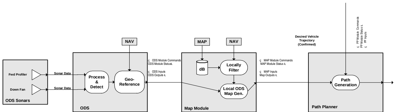
Fig. 9. System diagram of the OAS components of the AUTOTRACKER system.
