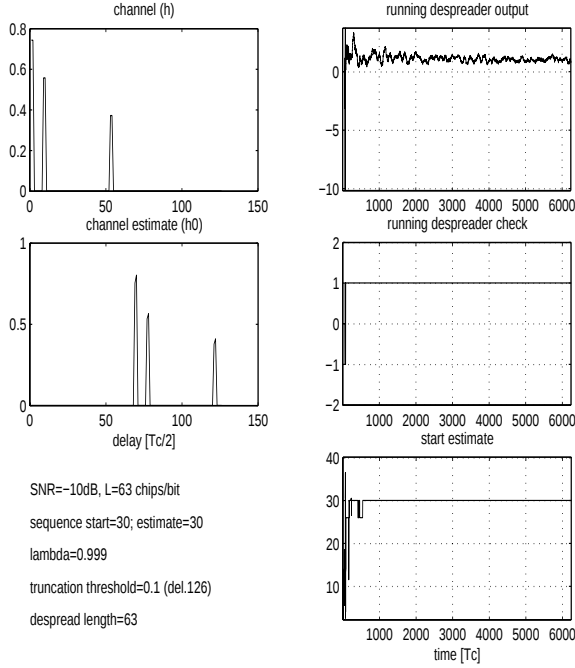
Fig. 1. Performance of the acquisition algorithm on the time-invariant AWGN channel.
