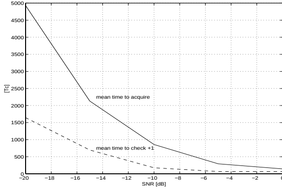
Fig. 3. Mean acquisition time for the 3-path time-invariant channel model.
