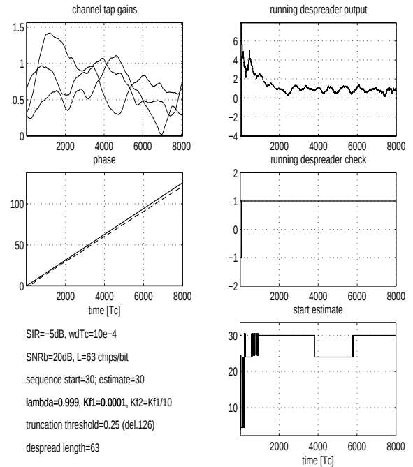
Fig. 4. Performance of the acquisition algorithm on a time-varying channel with four users. Each user's channel is an independent 3-path Rayleigh fading channel. Users move at different velocities (few m/s). Kasami sequences with randomly selected starting phase are used. The signals are of equal power and asynchronous.
