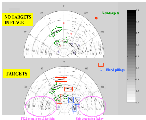
Fig. 2 Colorized plot of energy from the F122 ensouffed target field after WMF processing. Top panel is the no-target present condition while the bottom panel has the targets in place. Mine shapes are shown in red. Non-mine shapes are in green. Pink ovals indicate animal holding pens (left) and a ship degaussing facility (right).
