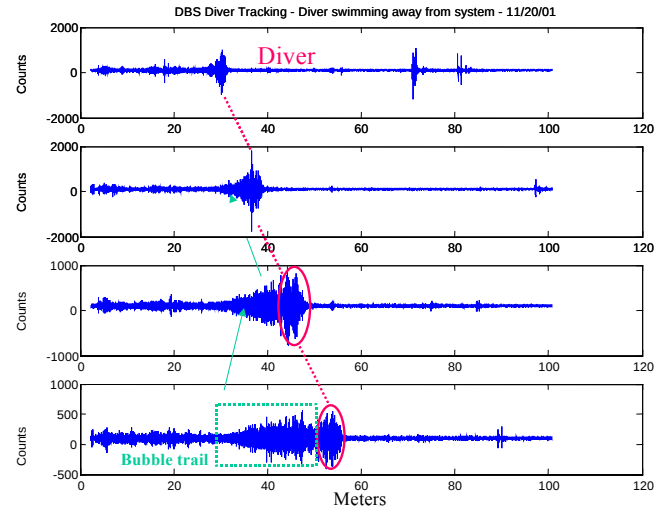
Fig.3 Diver swim path and resultant DBS backscatter from diver detection test.
