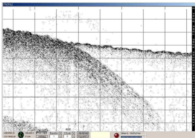
Fig. 16 An example of SBP data from the shallow water survey.
