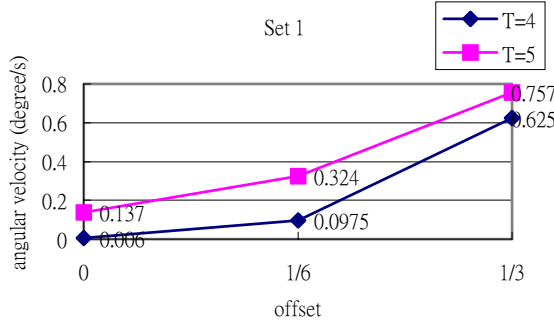
Fig. 13 The relation between offset and angular velocity
