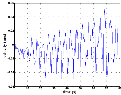
Fig. 26 The velocity in the y -direction
