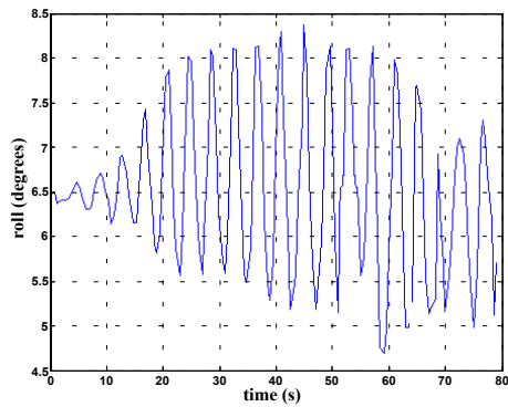
Fig.18 The roll of BAUV
