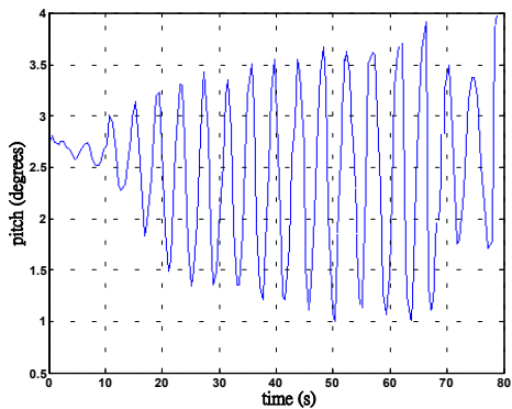
Fig. 19 The pitch of BAUV
