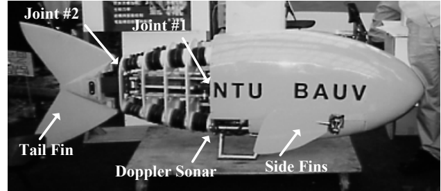
Fig. 1 Photograph of the testbed vehicle
