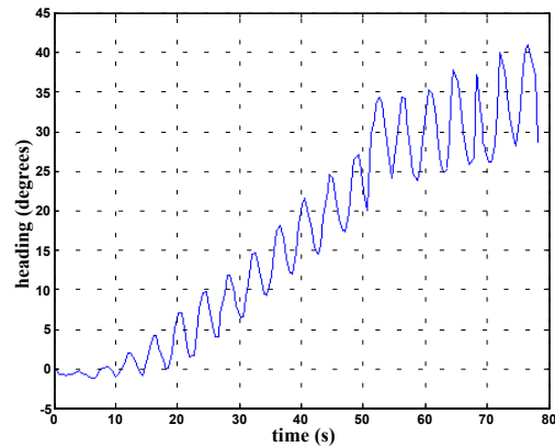
Fig. 17 The heading of BAUV
