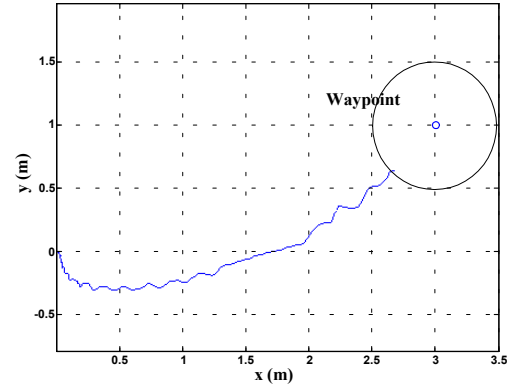
Fig. 16 The swimming path of BAUV, \lambda_e=2 , k_e=90
