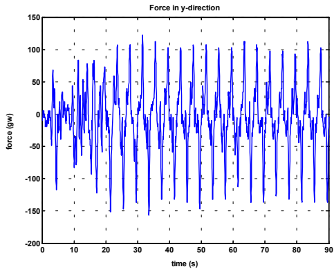
Fig. 8 The force in the y -direction
