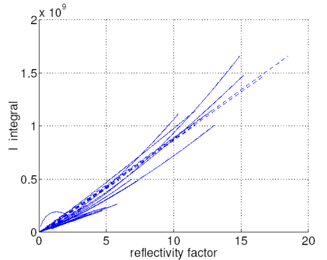
Fig 7. With the help of the same DSD models as before, I integral appearing in the expression of the surface elevation variance, versus the reflectivity factor. The dashed lines are obtained when the the Rayleigh approximation is used.
