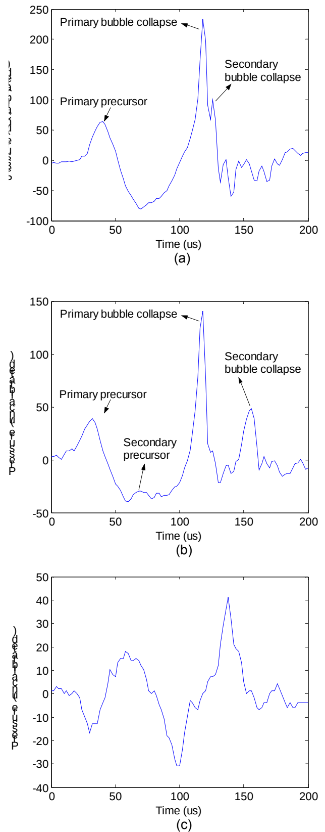
Fig. 8. Observed snaps at elevation angles of (a) 21.5^\circ , (b) 15^\circ and (c) 7.5^\circ
