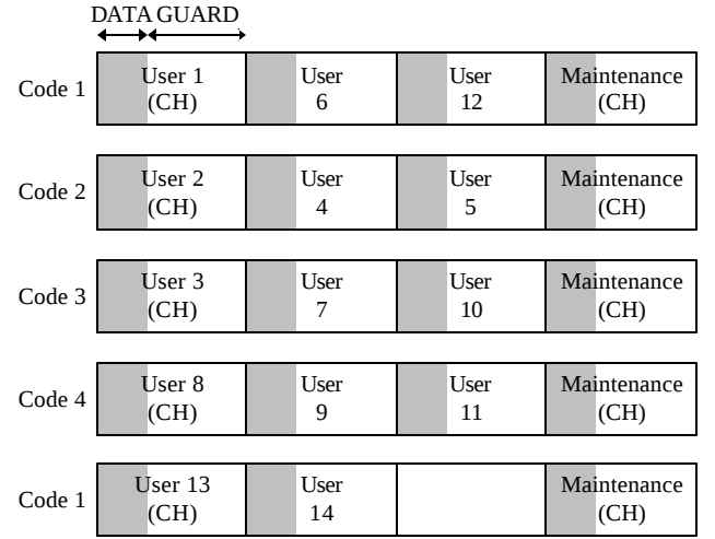
Fig. 2: Frame structure and code assignment. During slot 1, users 1, 2, 3, 8 and 13 transmit simultaneously.
