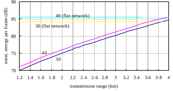
Fig. 9: Total (normalized) energy consumption per frame (25 km 2 , 6 nodes/cluster).
