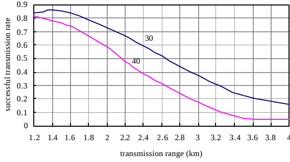
Fig. 12: Successful transmission rate (25 km 2 , 6 nodes/cluster).
