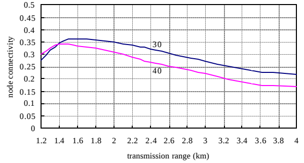
Fig. 10: Node connectivity (25 km 2 , 6 nodes/cluster).
