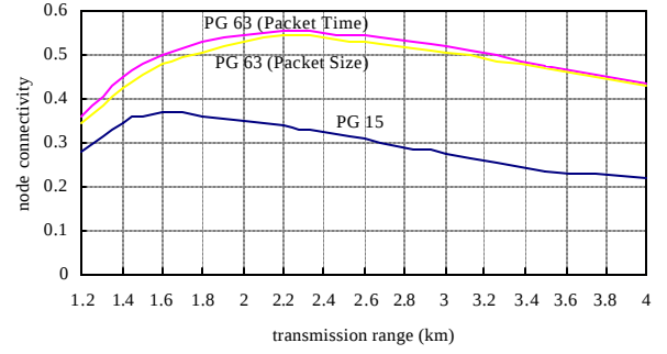
Fig. 14: Node connectivity for different processing gains.
