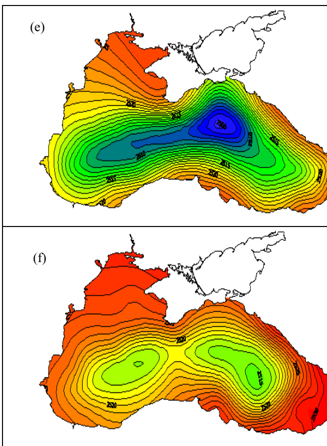
Fig.1 Climatic atlas map examples: (a) Temperature on 400 m; (b) Salinity on surface in May; (c) Density on 100 m in September; (d) Heat storage 0-100 m in September; (e) Dynamic height 0-300 db in February; (f) Dynamic height 0-300 db in August
