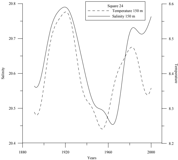
Fig. 3. Filtered Temperature and Salinity. Depth 150 m.
