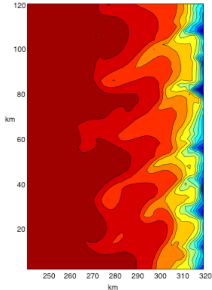
Fig. 7. Snapshot of SST on day 43 of the model run. Filaments curve southward, as they develop positive relative vorticity.
