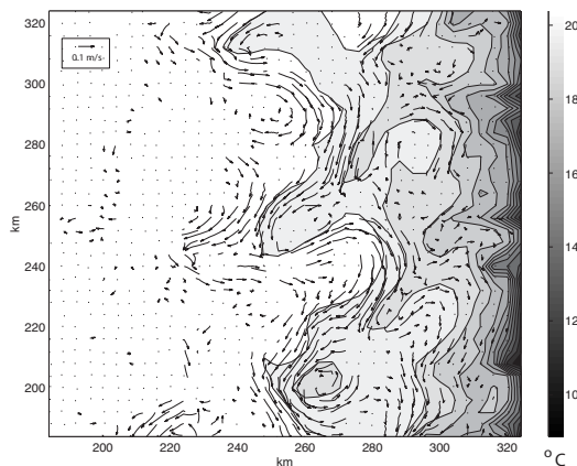
Fig. 4. Snapshot of SST (shading) and surface current (vectors) after 60 days of cooling.
