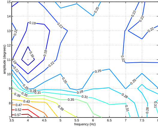
Fig. 9. Contour plot of efficiencies for all tests.
