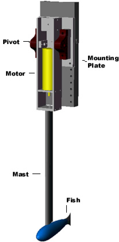
Fig. 2. Experimental Setup
