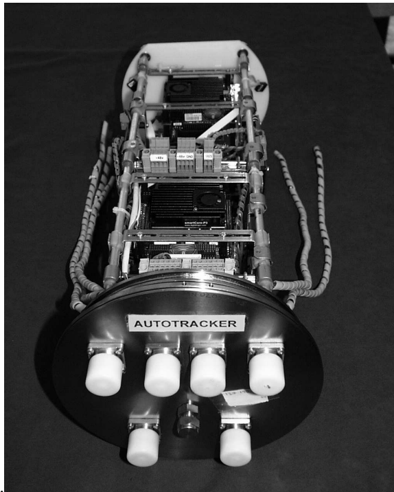
Figure 12: Photograph of the AUTOTRACKER "pod" – with its four high-performance PC104-based computers
