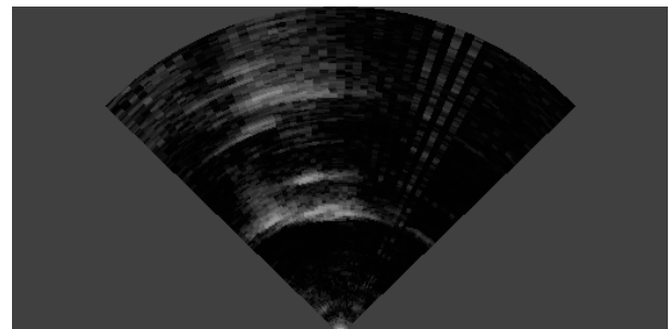
Figure 4: Typical SDS sonar image (panel @ 5m)
