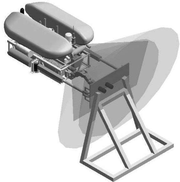
Figure 1: Illustration of the ALIVE AUV intervening with a standard ROV Docking Panel
