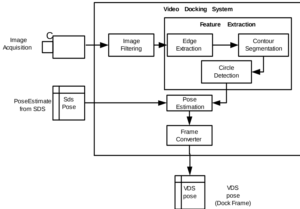
Figure 8: VDS (Video Docking System) Internal Architecture
