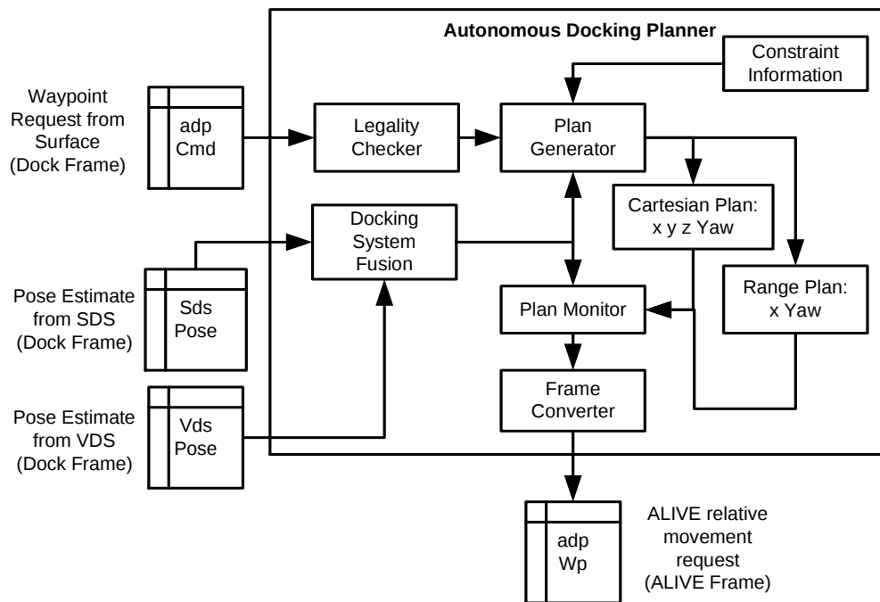
Figure 9: ADP (Autonomous Docking Planner) Internal Architecture
