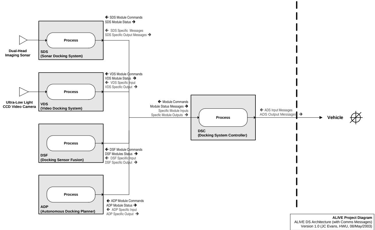
Figure 5: Overview of Autonomous Docking System (ADS) architecture for the ALIVE Intervention-AUV
