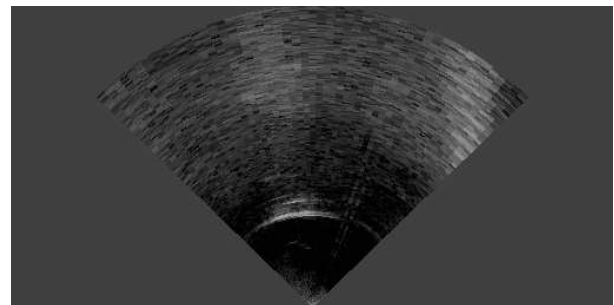
Figure 3: Typical SDS sonar image (panel @ 30m)
