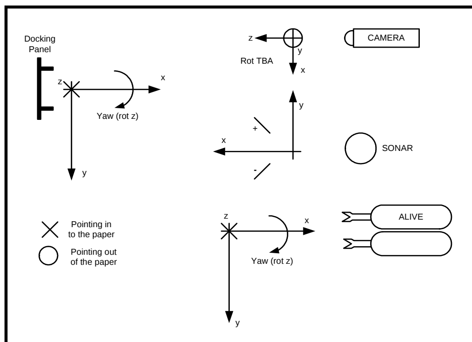
Figure 11: Various co-ordinates frames used within the ADP
