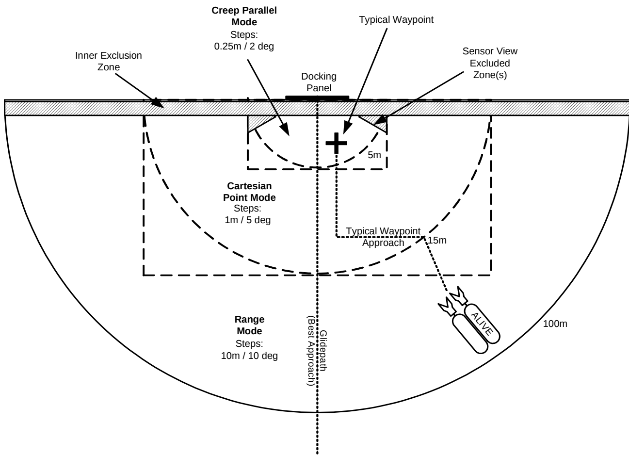
Figure 10: Operating modes of the ADP within the SLZ (Safe Landing Zone)
