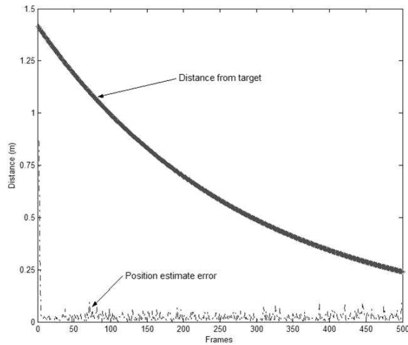
Figure 6: Typical VDS pose error at decreasing distance from target
