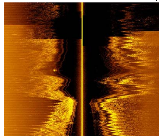
Figure 4: Image from CETUS II 2400 kHz with thrusters on vs. off
