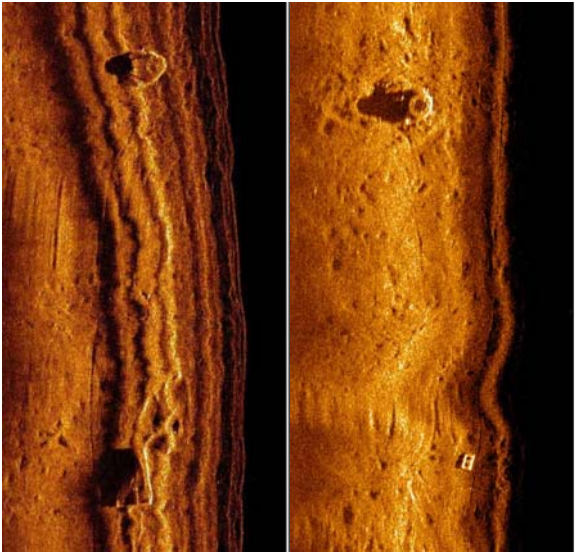
A. B. Figure 3: Beam Pattern Effects: A. shows a small vertical beam width (<20 degrees) with severe side lobes, while B. shows the effects of increasing the vertical beam width to ~30 degrees.
