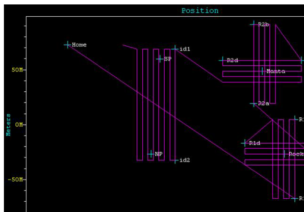
Figure 7: Typical path used for Reacquisition and Identification mission
