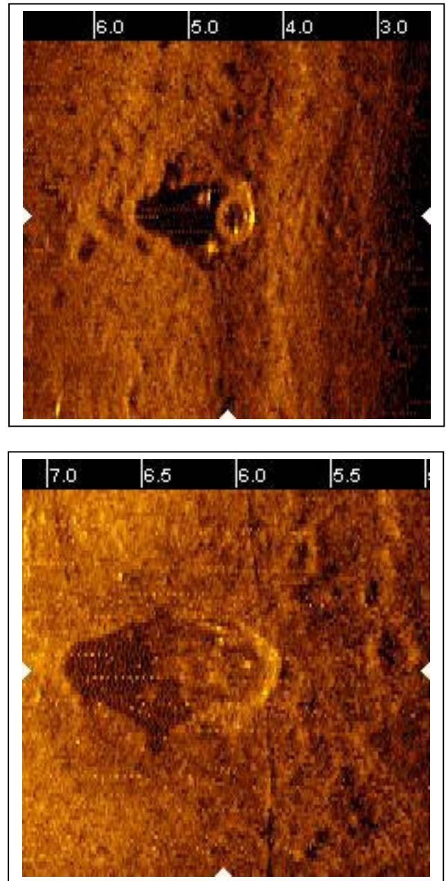
Figure 2: Images at 1200 kHz (top row) and 2400 kHz (bottom row)
