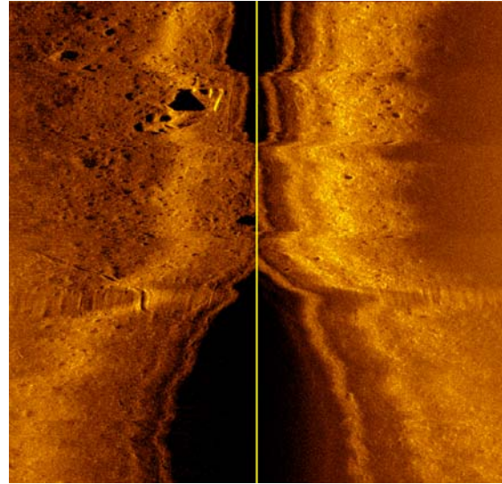
Figure 6: Image from 2400 kHz at 3.2 knots
