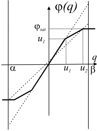
Figure 5: Static input nonlinearity.
