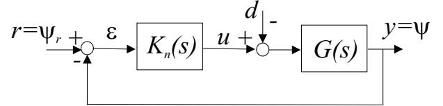
Figure 6: Nominal closed loop control problem.
