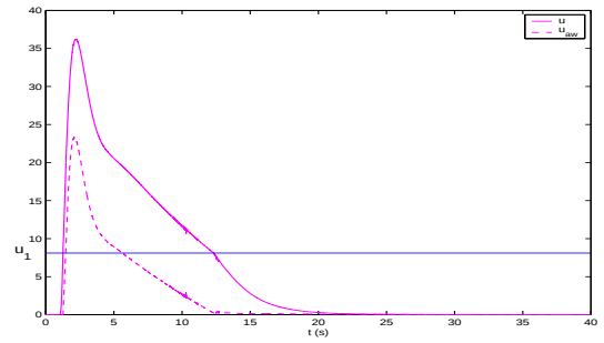
Figure 16: Control signals u and u_{aw} step response.
