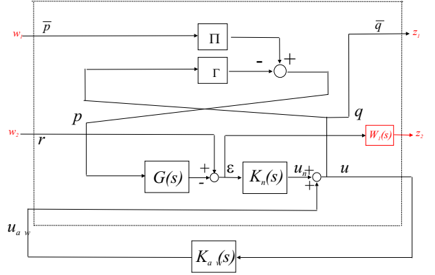
Figure 12: K_{aw} synthesis problem: an \mathbf{H}_\infty standard representation.
