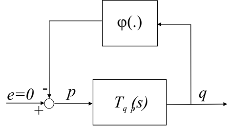
Figure 4: Linear system and a nonlinear interconnection.
