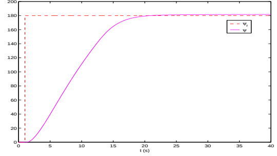
Figure 15: Heading \psi step response.
