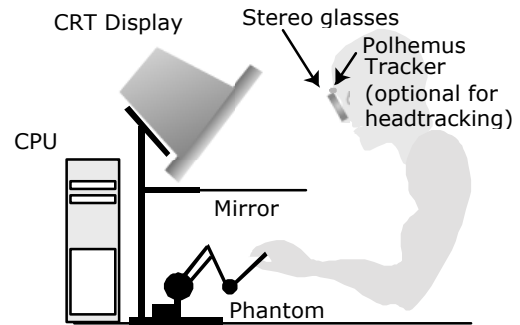
Figure 1. Haptic Fish Tank setup.
