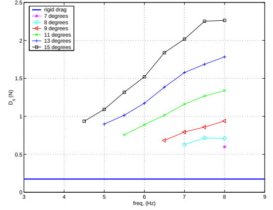
Fig. 12. Upper bound estimate of D_s .
