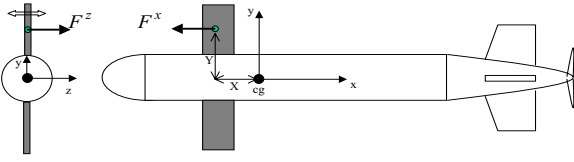
Fig. 1. Schematic of a BAUV with one pair of pectoral fins
