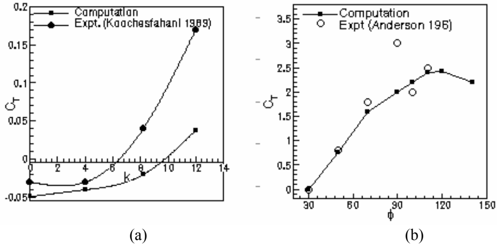
Figure 13. Comparison between simulations (Ramamurti et al.) and experiments (Koochesfahani [48]) and Anderson [7]. (a) Effect of frequency parameter for pitch oscillations of 2^\circ at Re=1.2 \times 10^4 . (b) effect of phasing between pitch and plunge motion for k=3.8 and Re=1.1 \times 10^3 .
