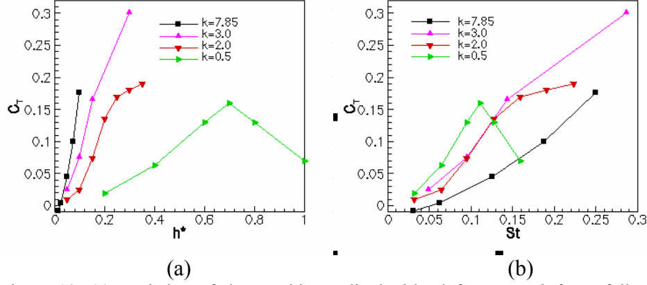
Figure 10. (a) Variation of thrust with amplitude h^* and frequency k for a foil undergoing plunge oscillations as computed by Tuncer & Platzter [15]. (b) Data replotted using Strouhal number (St) shows better collapse.
