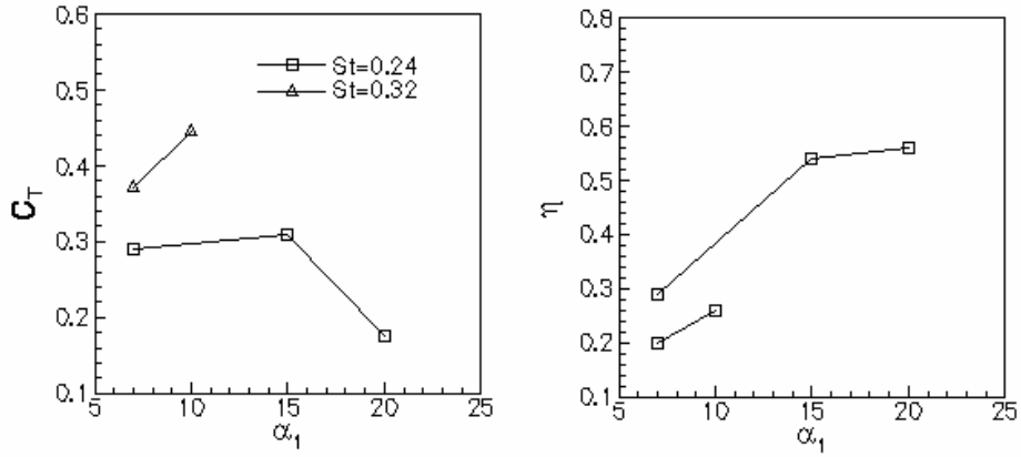
Figure 11. Effect of pitch amplitude and Strouhal number on thrust for airfoil undergoing combined pitch and heave. ( h_1^* = 0.75 , \phi = 75^\circ ). Results from computations of Tuncer & Platzter [15]
