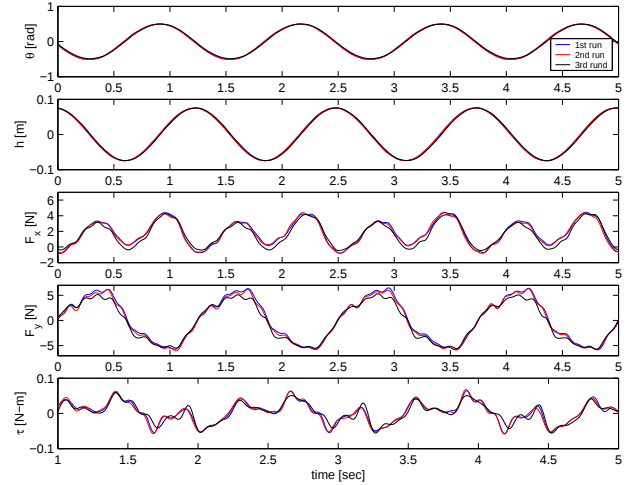
Fig. 18. The time traces of pitch and heave positions, instantaneous thrust and lift forces, and applied torque for the rigid foil, with the simple harmonic motion profile, when St = 0.3 and \alpha = 15^\circ .
