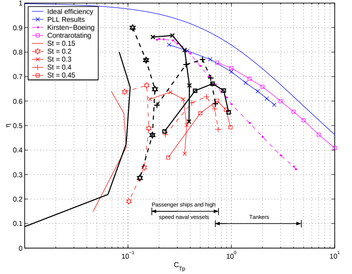
Fig. 17. The propulsive efficiency as function of the C_{Tp} , using harmonic angle of attack profile, for different Strouhal numbers. The thick and thin lines represent the results from Shore A60 and rigid foil, respectively.
