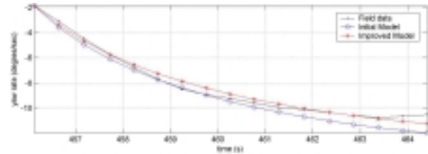
Figure 8: Yaw model improvements, +15^\circ rudder
