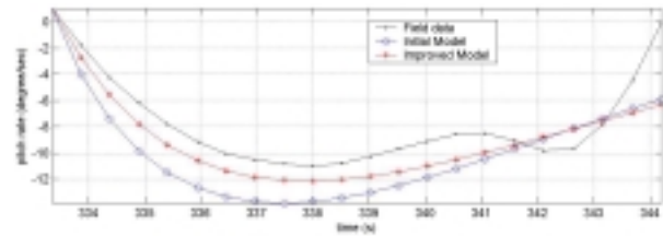
Figure 9: Pitch model improvements, +15^\circ elevator
