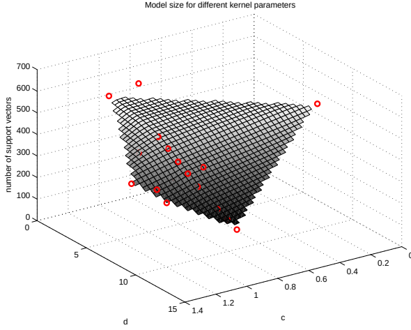
Figure 8: Average model size for 8-fold cross-validation of SVMs trained on our test data using various kernel parameters. Circles indicate particular model parameters tried. The fact that model size correlates well with error rate indicates that the models are too restrictive and not over-fitted. The smallest model so far contains 233 support vectors.
