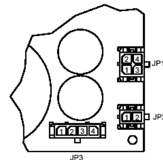
202004 Power Amp RFF Connector Pinout
