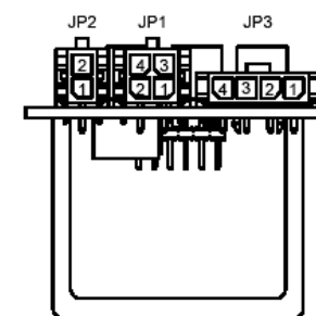
202001 Power Amp LFF Connector Pinout
